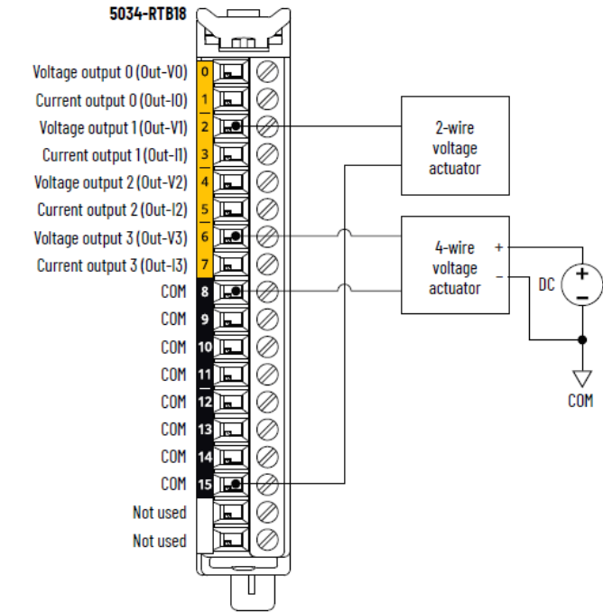
Figure 33. 5034-OF4 and 5034-OF4XT Wiring Diagram – Voltage Mode
