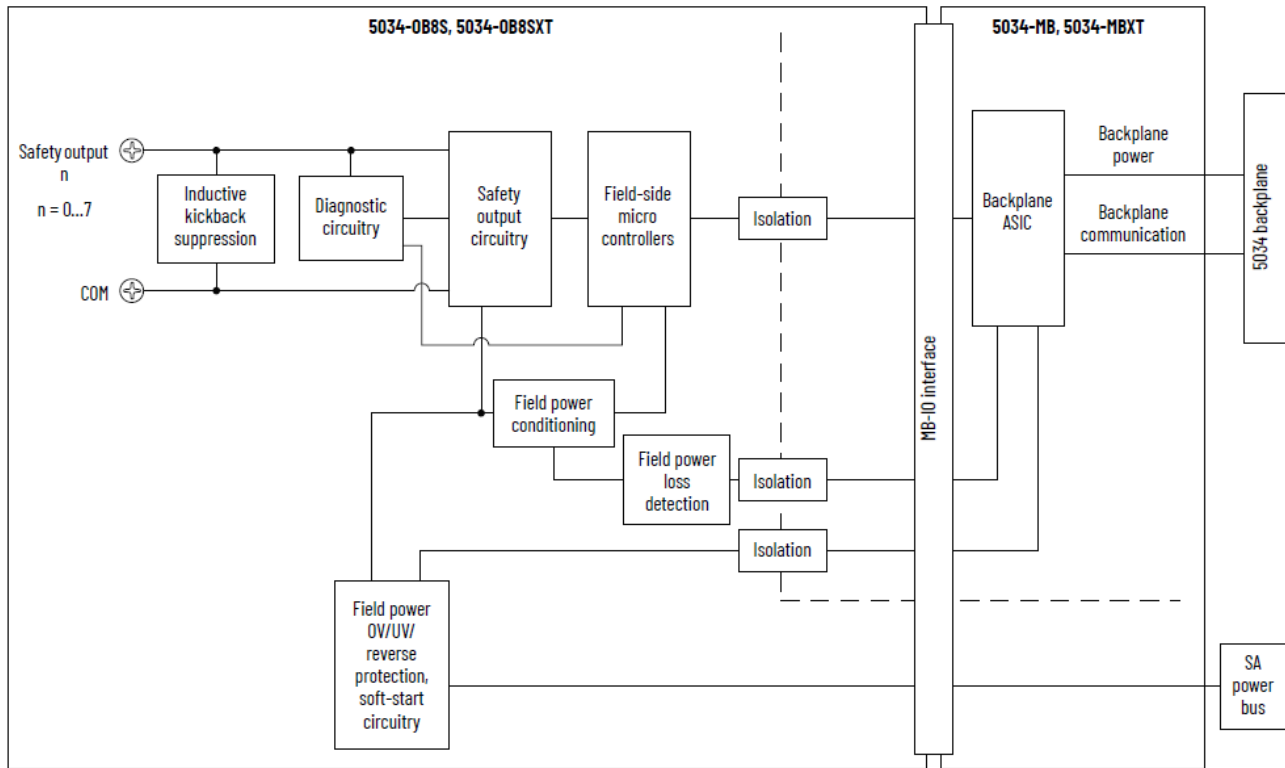
Figure 21. 5034-0B8S and 5034-0B8SXT Functional Block Diagram
