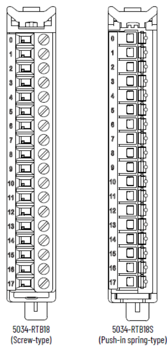
Figure 43. 5034-RTB18 and 5034-RTB18S Diagram
