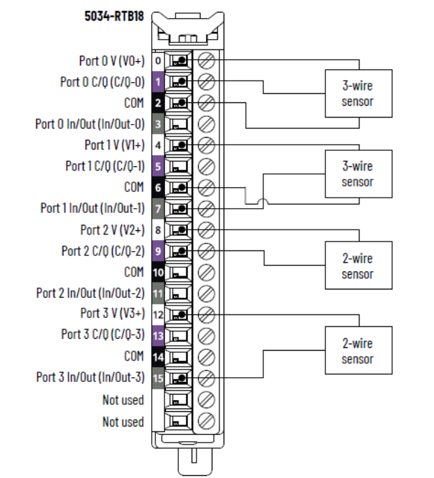
Figure 36. 5034-IOL4 and 5034-IOL4XT Wiring Diagram – DI Mode
