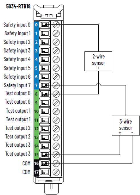
Figure 18. 5034-IB8S and 5034-IB8SXT Wiring Diagram - 2-wire and 3-wire Sensor Wiring
