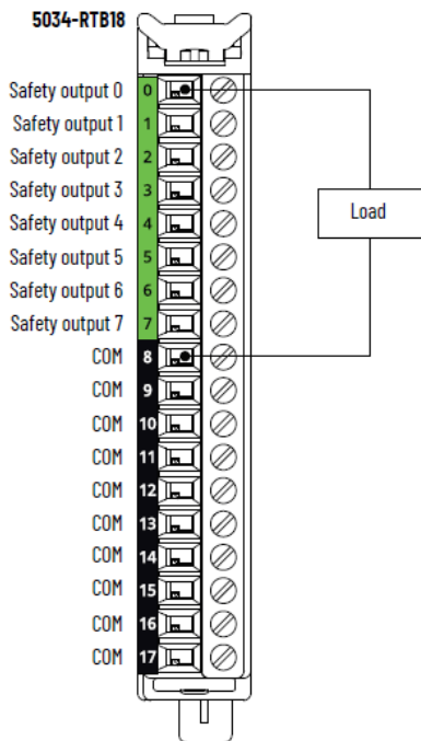
Figure 20. 5034-OB8S and 5034-OB8SXT Wiring Diagram
