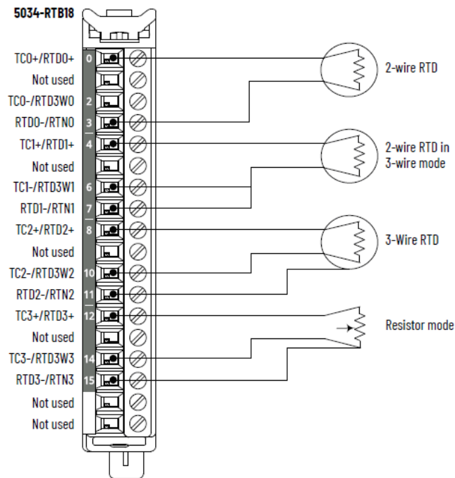
Figure 29. 5034-IRT4I and 5034-IRT4IXT Wiring Diagram - RTD Mode
