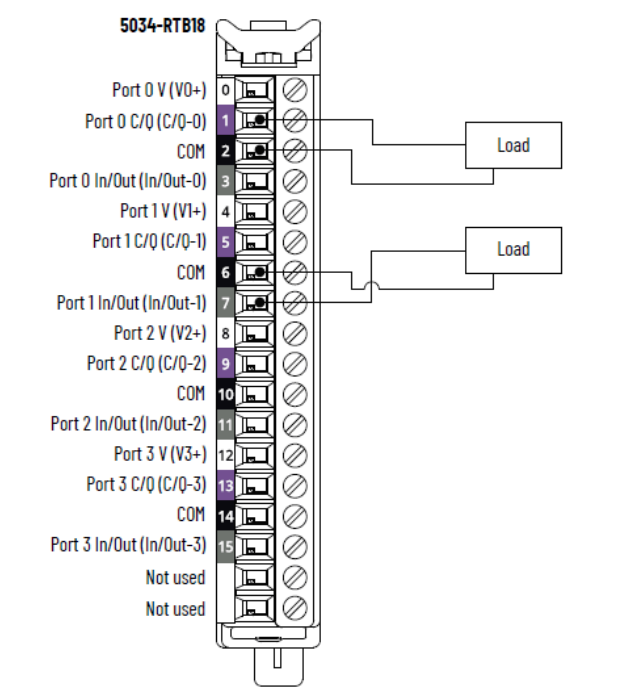
Figure 37. 5034-IOL4 and 5034-IOL4XT Wiring Diagram – DO Mode
