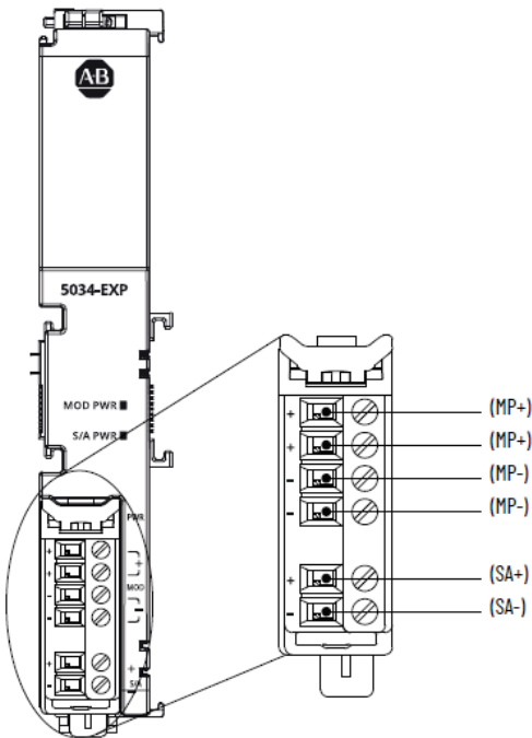
Figure 39. 5034-EXP and 5034-EXPXT Diagram
