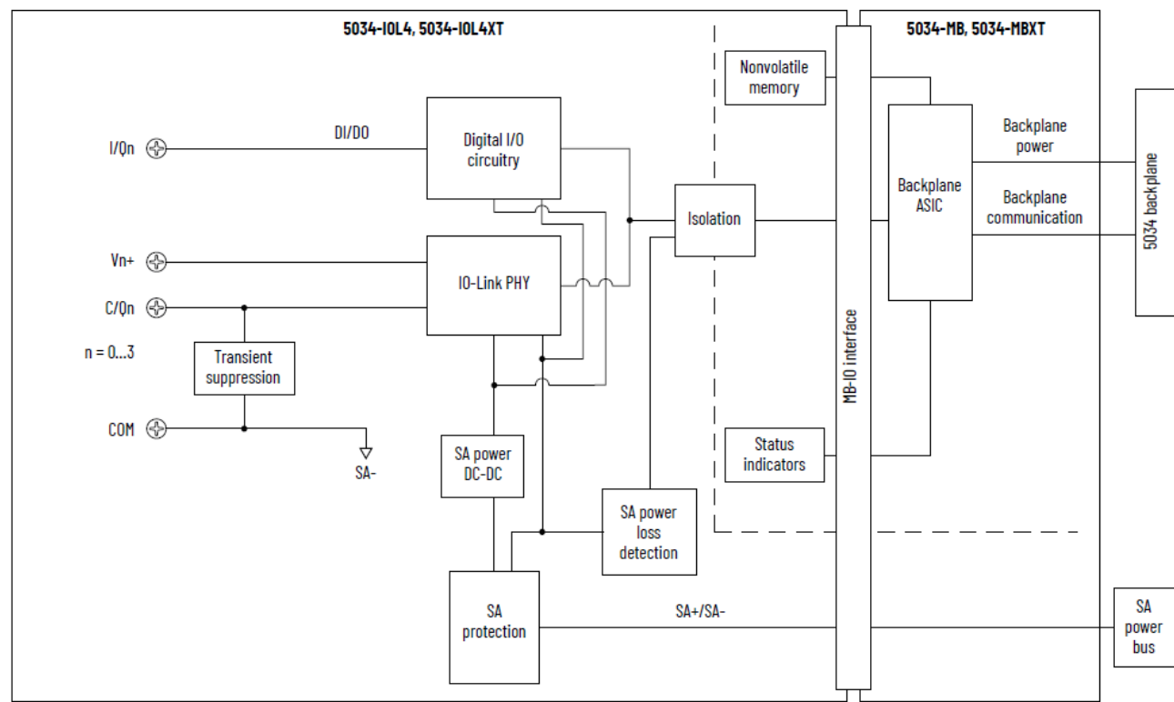
Figure 38. 5034-IOL4 and 5034-IOL4XT Functional Block Diagram
