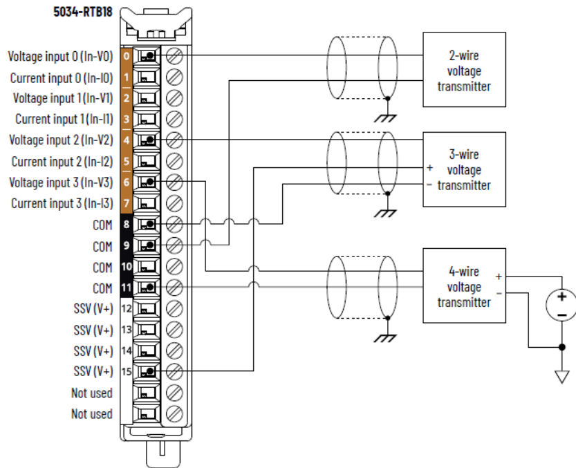
Figure 27. 5034-IF4 and 5034-IF4XT Wiring Diagram - Voltage Mode
