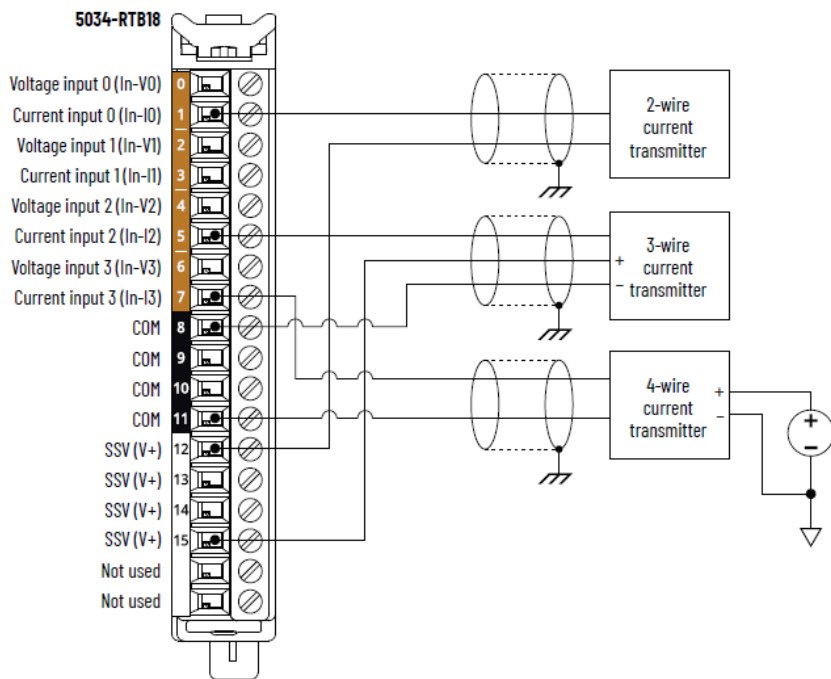
Figure 26. 5034-IF4 and 5034-IF4XT Wiring Diagram - Current Mode
