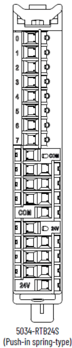
Figure 44. 5034-RTB24S Diagram
