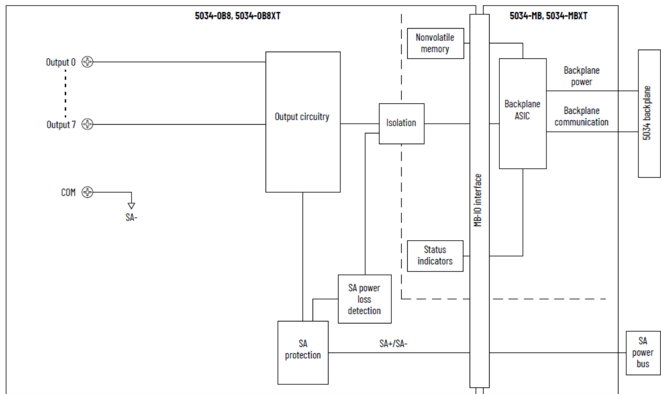
Figure 15. 5034-OB8 and 5034-OB8XT Functional Block Diagram
