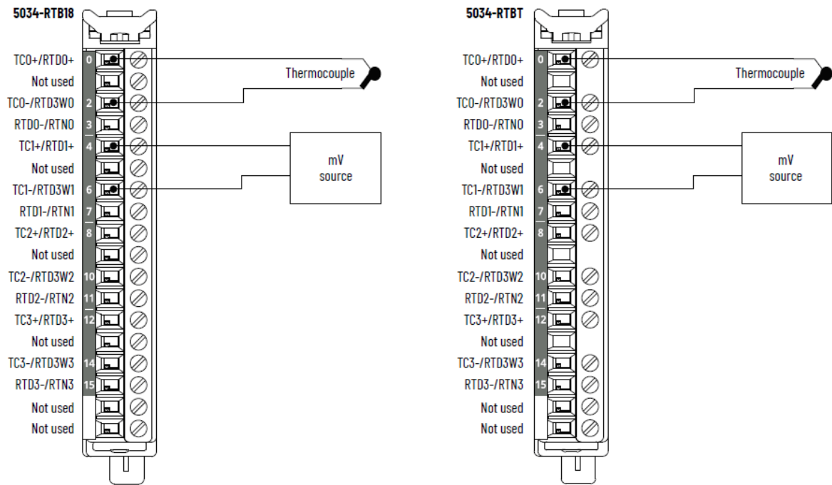
Figure 30. 5034-IRT4I and 5034-IRT4IXT Wiring Diagram - Thermocouple Mode
