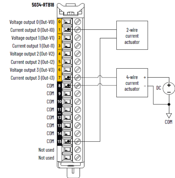
Figure 32. 5034-OF4 and 5034-OF4XT Wiring Diagram – Current Mode
