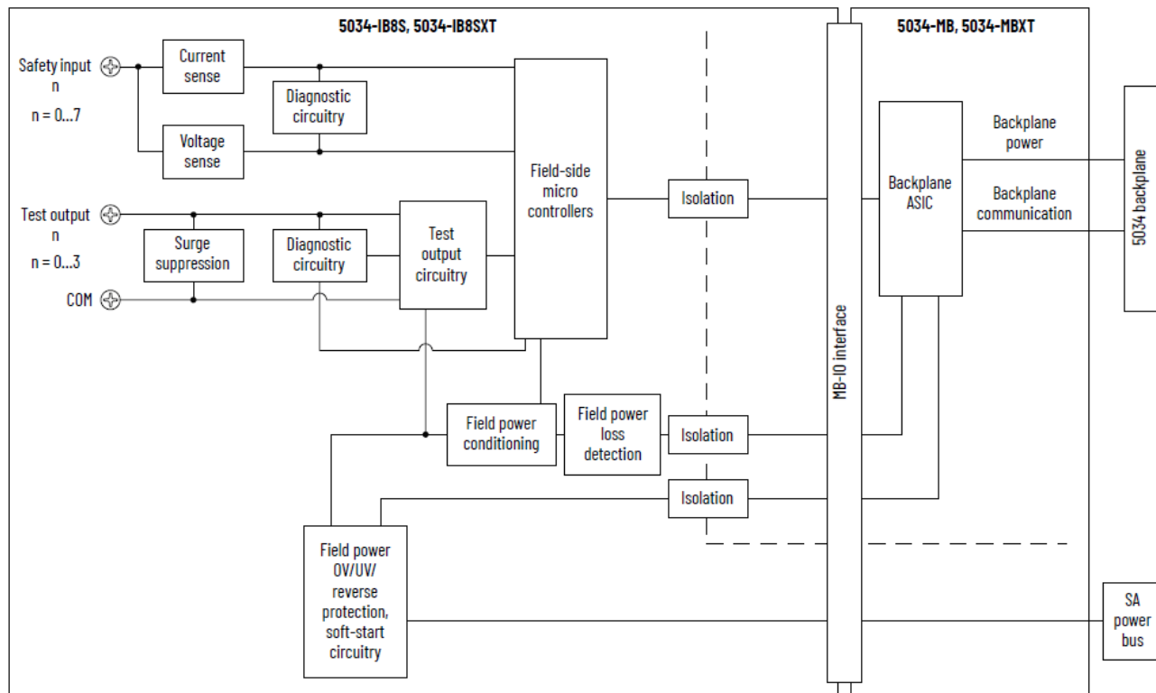
Figure 19. 5034-IB8S and 5034-IB8SXT Functional Block Diagram
