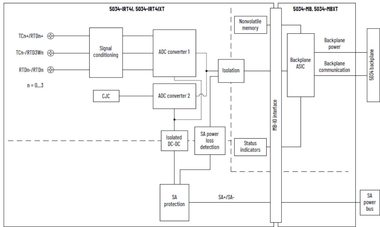
Figure 31. 5034-IRT4I and 5034-IRT4IXT Functional Block Diagram
