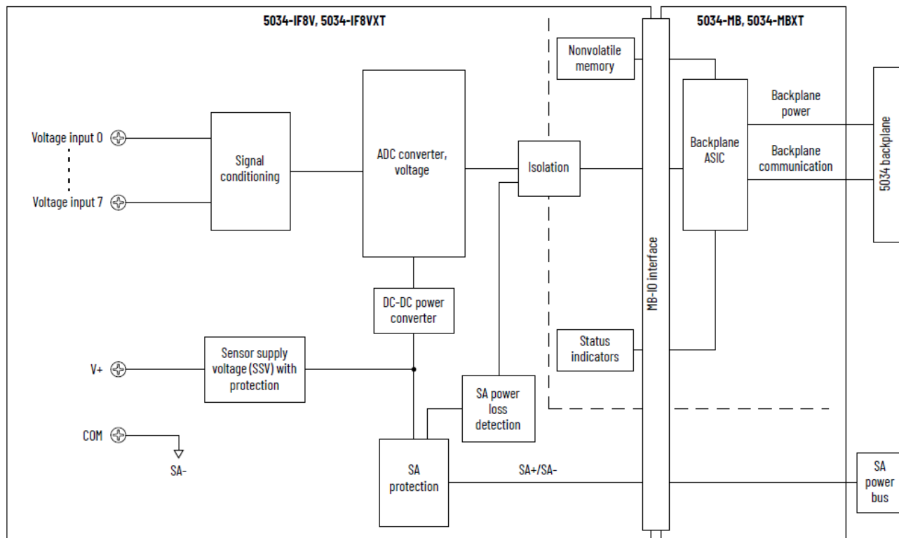
Figure 25. 5034-IF8V and 5034-IF8VXT Functional Block Diagram
