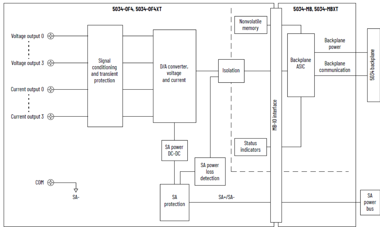
Figure 34. 5034-OF4 and 5034-OF4XT Functional Block Diagram
