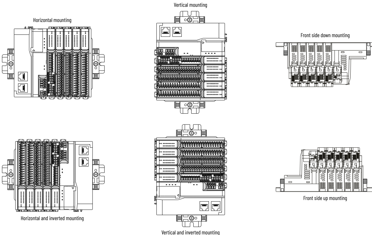
Figure 2. PointMax I/O System Mounting Orientations
