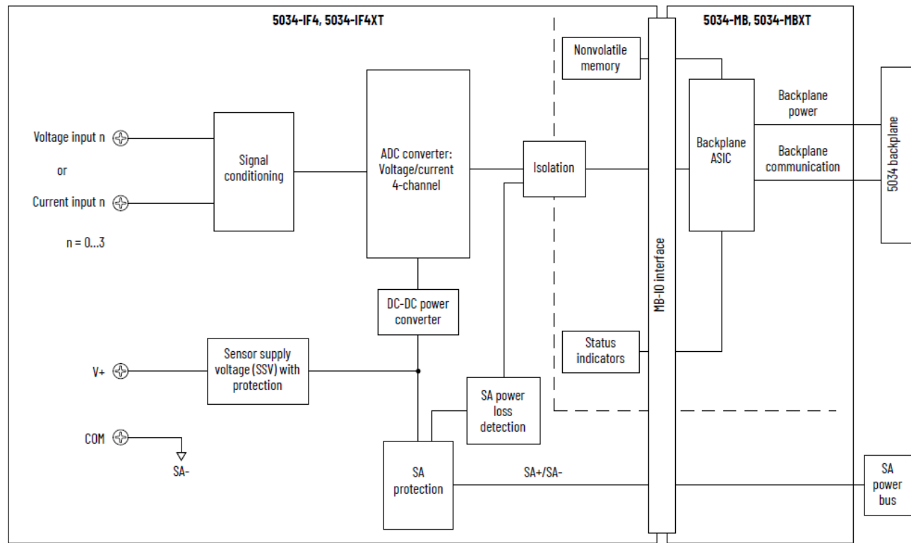
Figure 28. 5034-IF4 and 5034-IF4XT Functional Block Diagram
