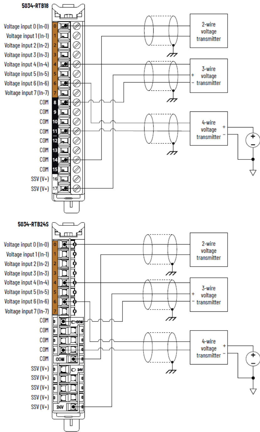
Figure 24. 5034-IF8V and 5034-IF8VXT Wiring Diagram
