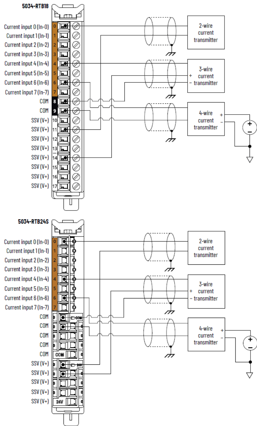
Figure 22. 5034-IF8C and 5034-IF8CXT Wiring Diagram
