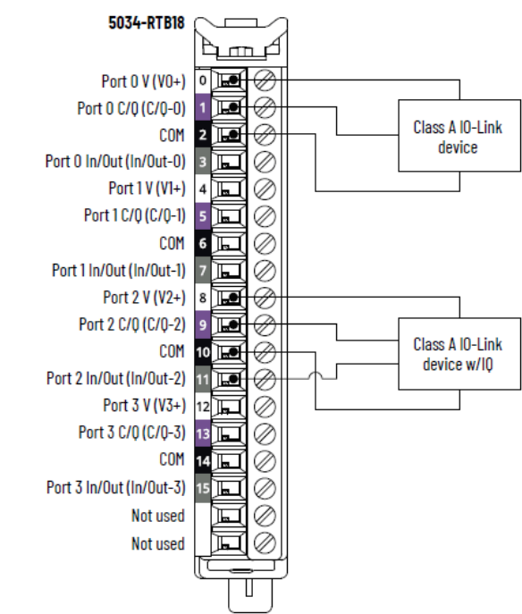
Figure 35. 5034-IOL4 and 5034-IOL4XT Wiring Diagram – IO-Link Mode
