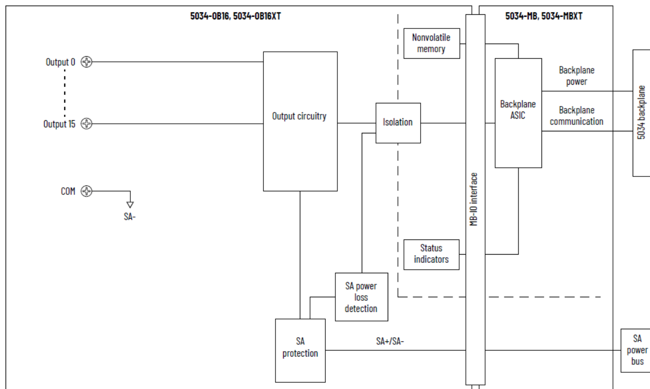
Figure 13. 5034-OB16 and 5034-OB16XT Functional Block Diagram
