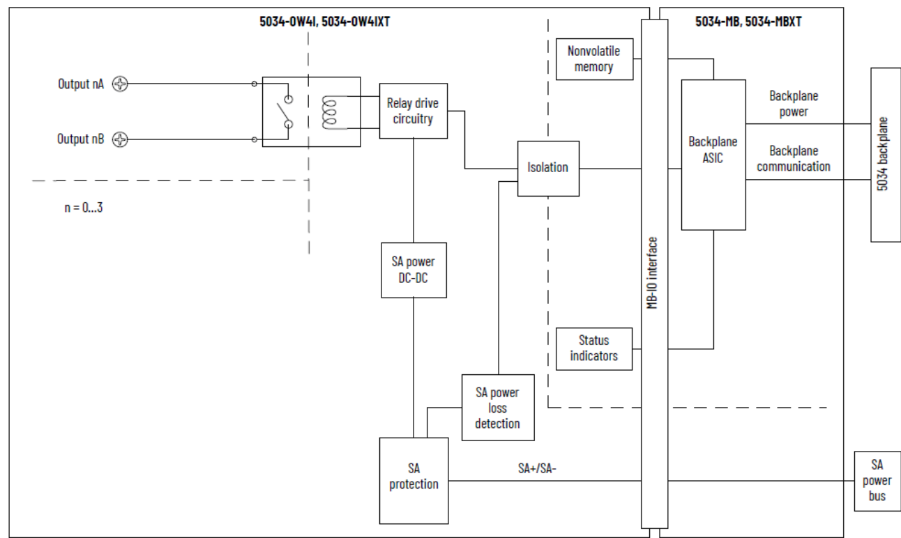
Figure 17. 5034-0W4I and 5034-0W4IXT Functional Block Diagram
