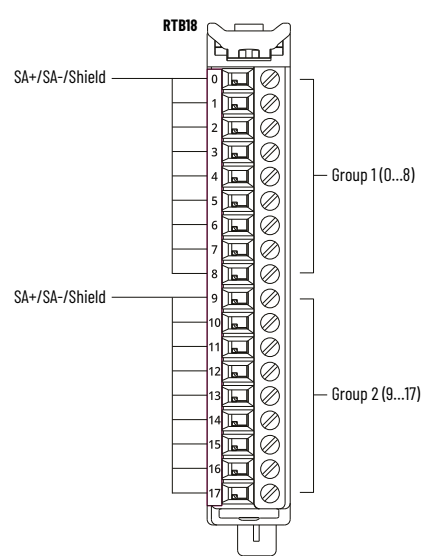
Figure 40. 5034-MBPTM and 5034-MBPTMXT Wiring Diagram
