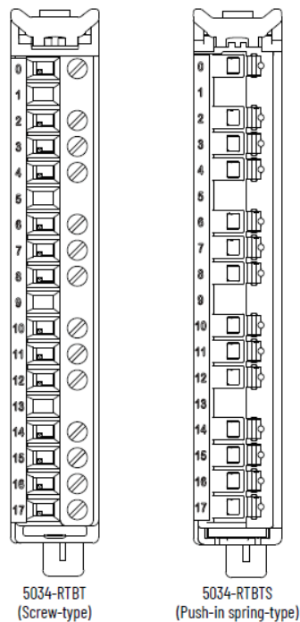
Figure 45. 5034-RTBT and 5034-RTBTS Diagram
